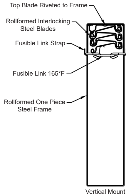
Vertical Mount
